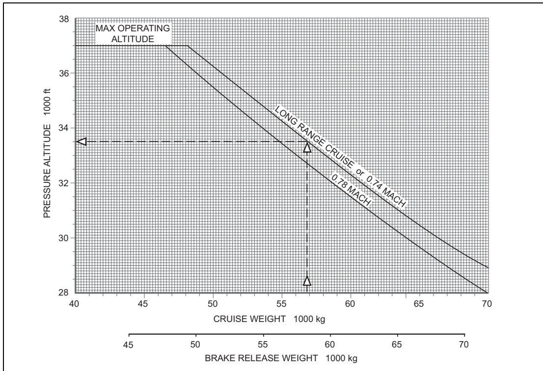
Figure 4.1 Optimum Altitude
